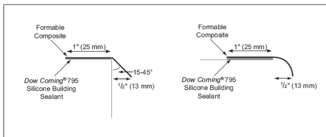
Figure 1: Drip Edge Design
