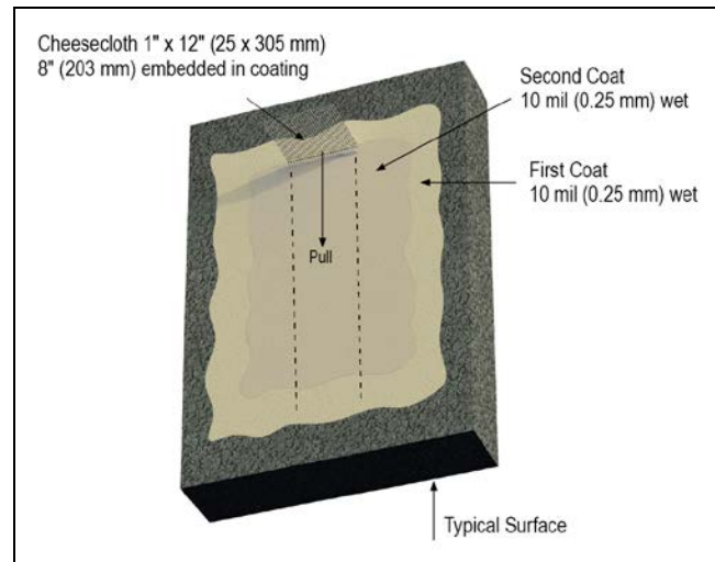
Figure 2: Test Procedure Diagram
